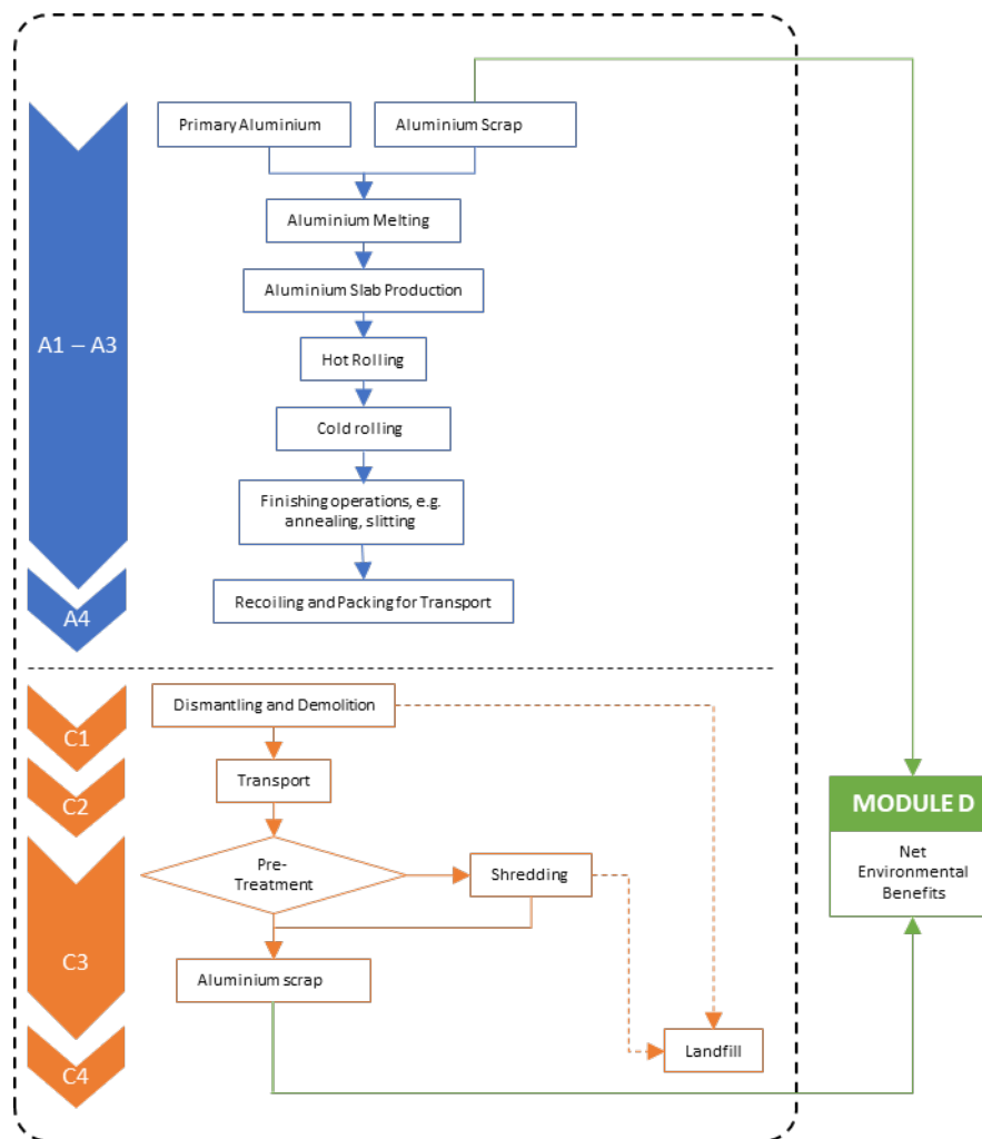
Figure 1 Main production processes and components of the Aluminium sheet
