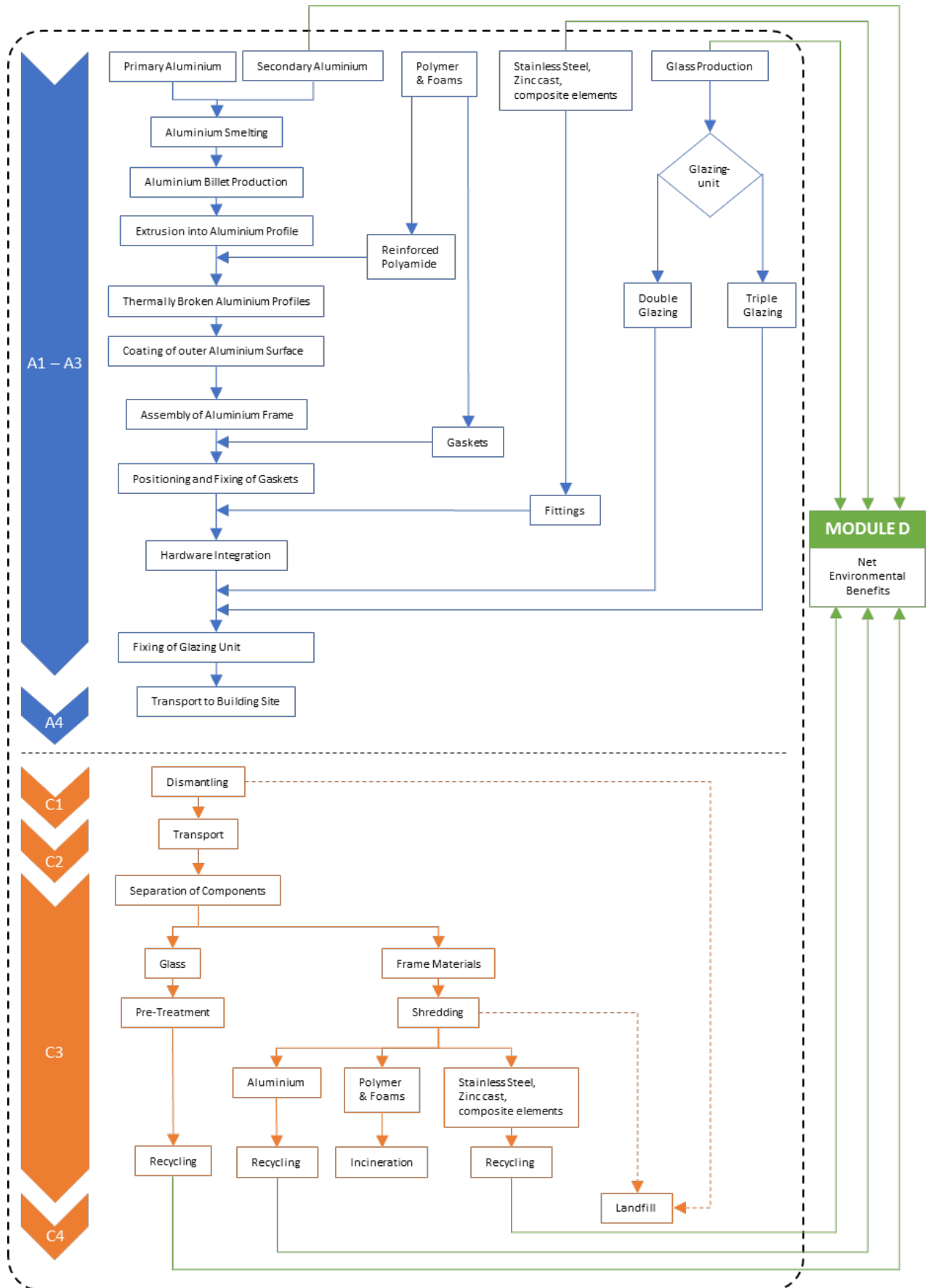
Figure 1 Main production processes and components of the go-to sliding system
