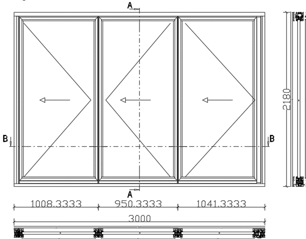
Figure 1 Sketch of the representative product for the insulated folding door
