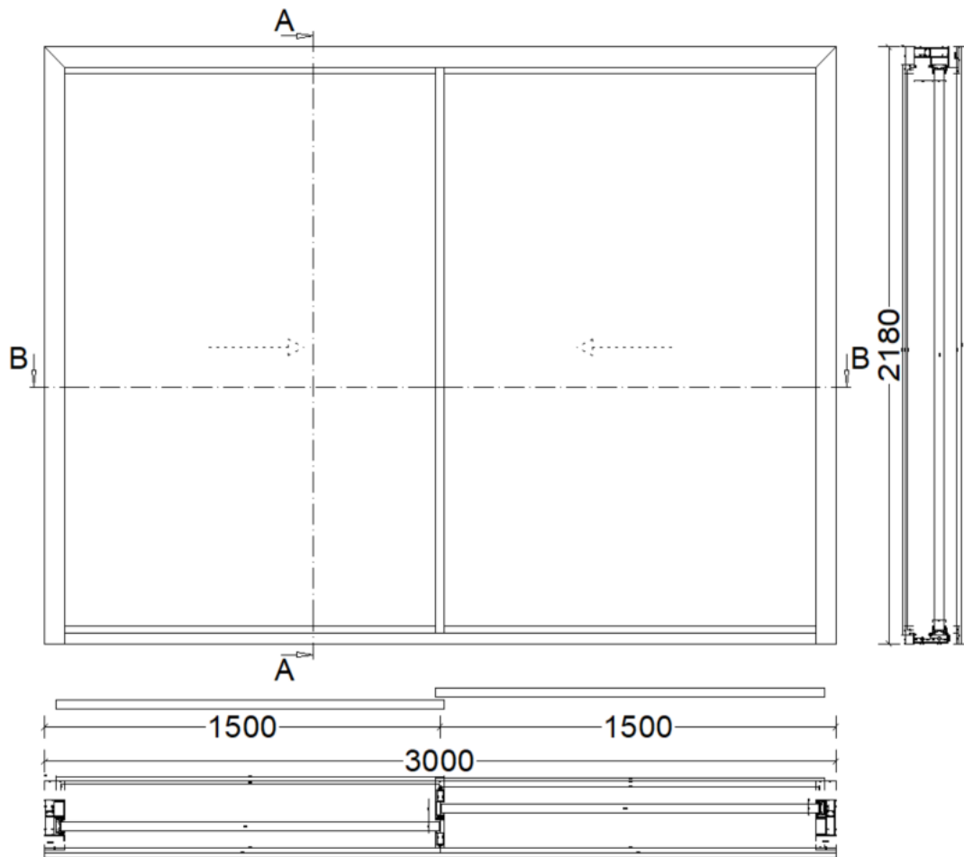
Figure 1 Sketch of the representative product for the minimal sliding door
