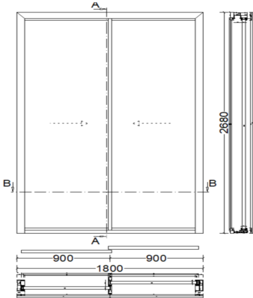
Figure 2 Sketch of the representative product for the minimal sliding door
