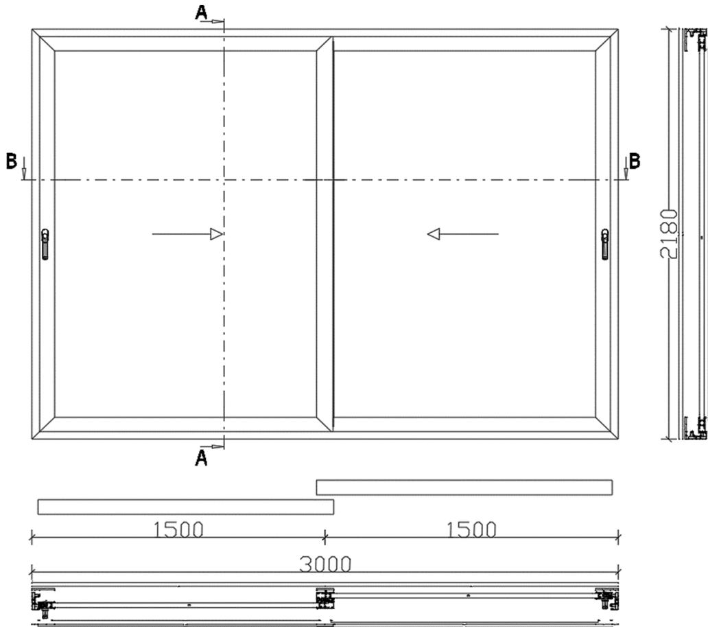
Figure 1 Sketch of the representative product for the sliding non insulated system
