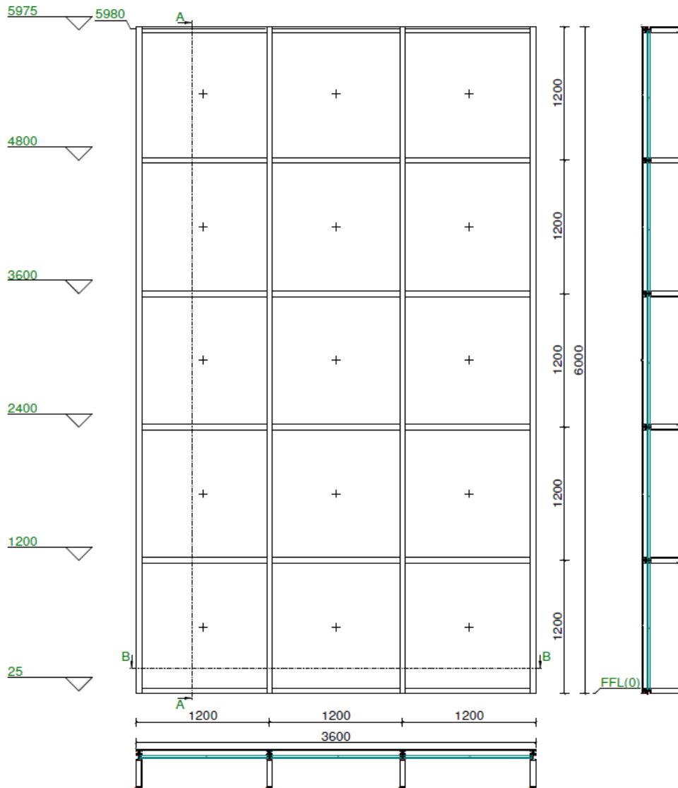
Figure 1. Sketch of the representative product for the M50 curtain wall.
